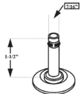
-11- GRIP RING STEM
