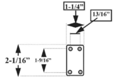
-01- TOP PLATE
