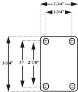
-01- TOP PLATE
