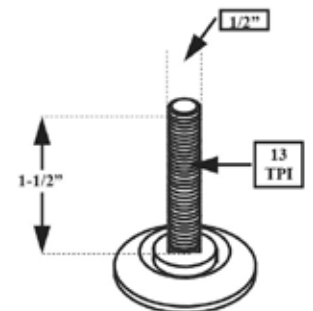
-21- THREADED STEM
