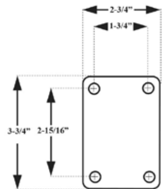
-01- TOP PLATE
